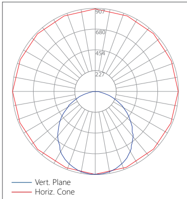
Relative Luminous Intensity RLK G2 T22
