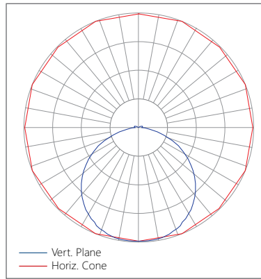
Relative Luminous Intensity with CA lens
